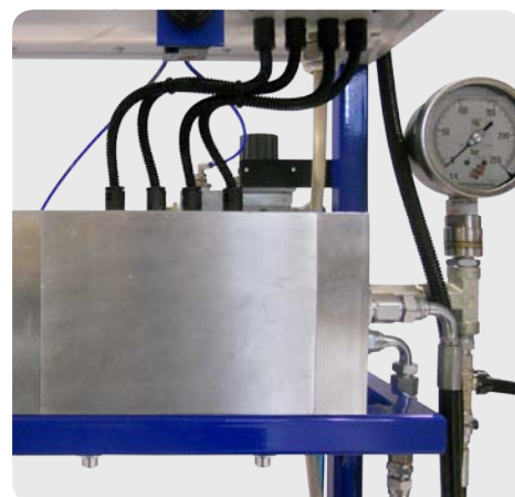
HEAT EXCHANGER AND OVERPRESSURE GAUGE
